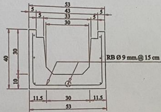
CROSS SECTION
